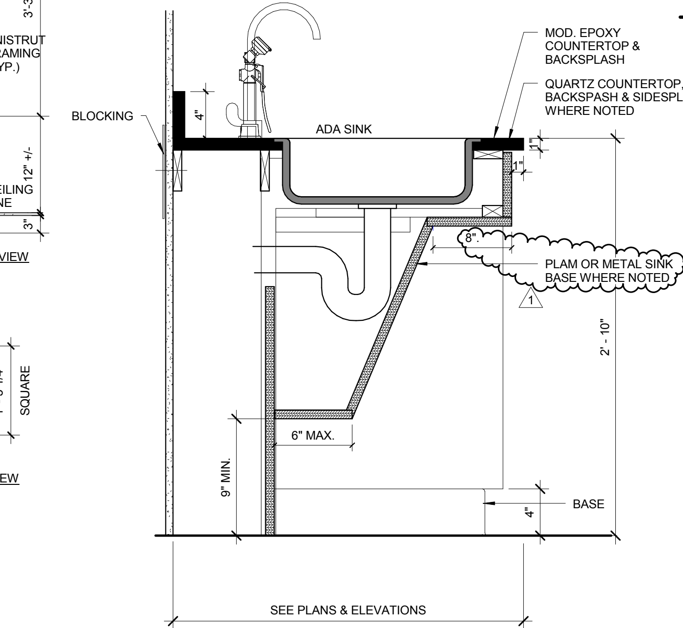
4 ADA SINK DETAIL W/O POCKET DOORS 1 1/2" = 1'-0"
