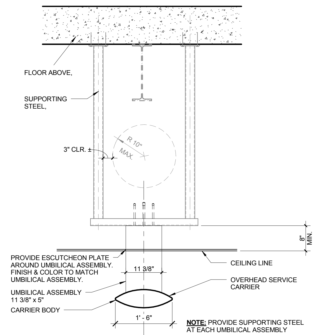
10 OSC MOUNTING DETAIL 3/4" = 1'-0"
