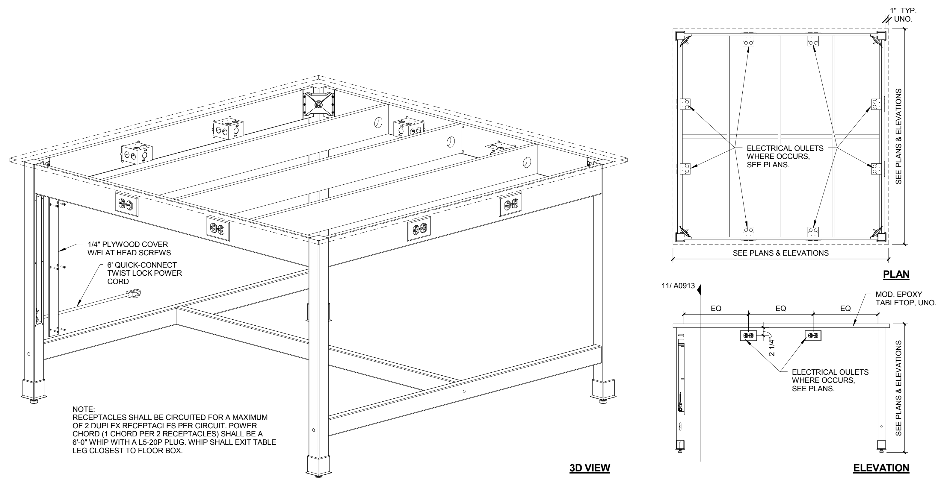
12 TABLE WITH ELEC. OUTLETS ON APRON 3/4" = 1'-0"
