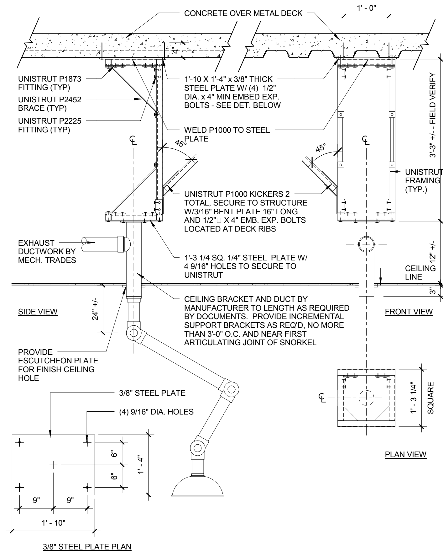
5 SNORKEL EXHAUST MOUNTING DETAIL 3/4" = 1'-0"
